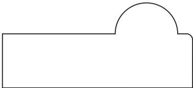
HWP8133 Molding 0.875" x 1.937"
