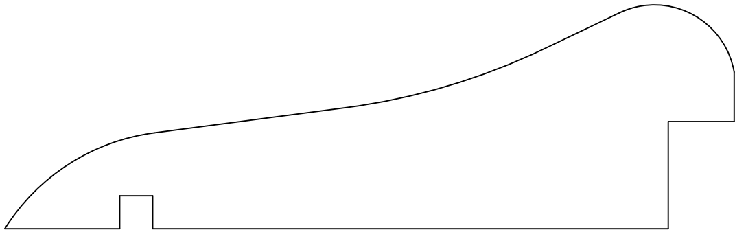
HWP7790 Rail 1.687" x 5.531"
