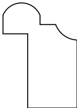
HWP7662 Molding 1.062" x 0.750"
