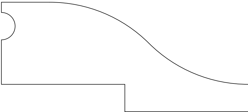
HWP7654 Molding 2.000" x 4.500"
