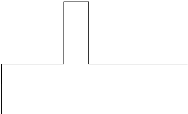
HWP7640 Molding 2.250" x 3.750"
