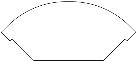
HWP7629 Quarter Round 1.250" x 2.840"
