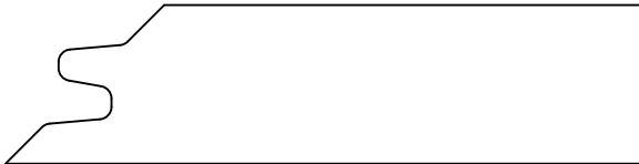
HWP7558 Lock Miter 0.750 x 3.000
