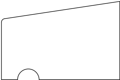
HWP7477 Molding 2.062" x 1.375"
