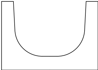
HWP7423 Molding 1.250" x 1.750"
