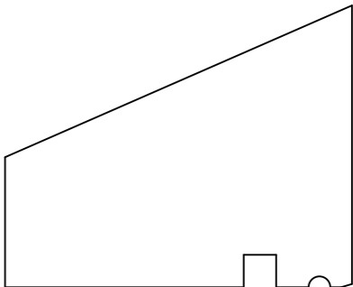
HWP7412 Molding 0.750" x 1.625"
