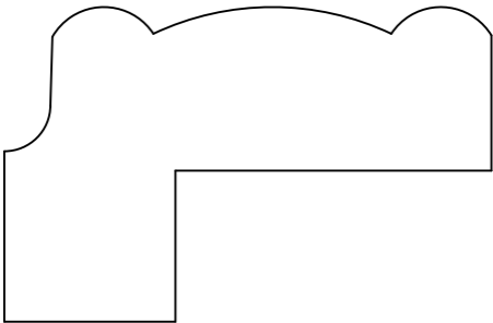
HWP7391 Molding 1.500" x 2.312"
