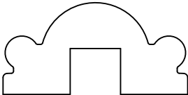
HWP7359 Molding 0.687" x 1.375"
