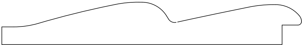
HWP5512 Planking 0.750" x 5.250"
