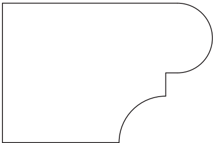
HWP4875 Nosing 1.500" x 2.250"
