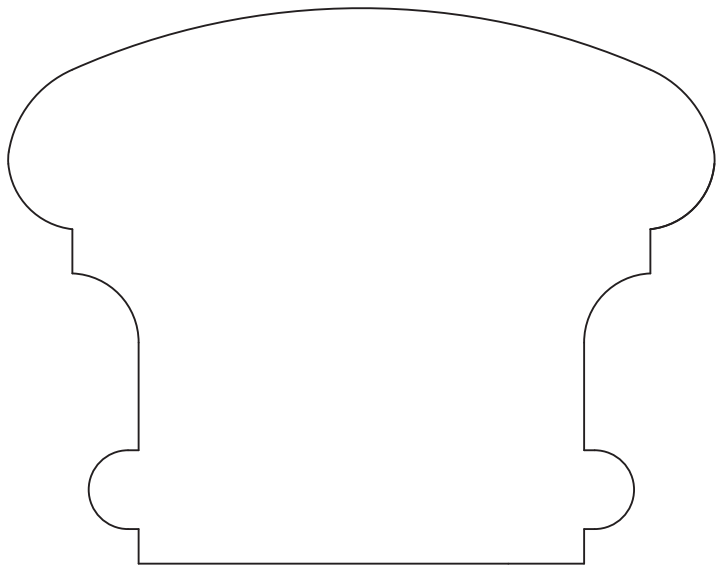
HWP4712 Handrail 2.890" x 3.680"
