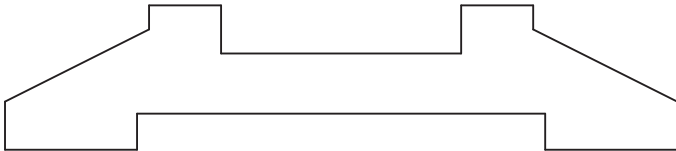
HWP4711 Handrail Shoe 0.750" x 3.500"
