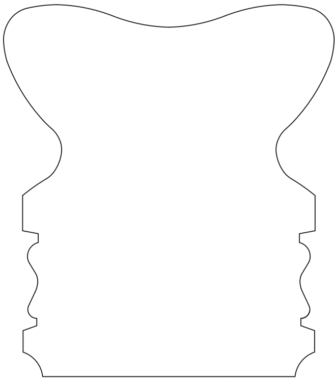
HWP4708 Handrail 3.800" x 3.380"
