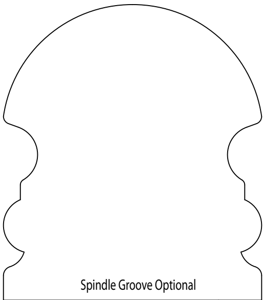
HWP4550 Handrail 3.000" X 2.625"
