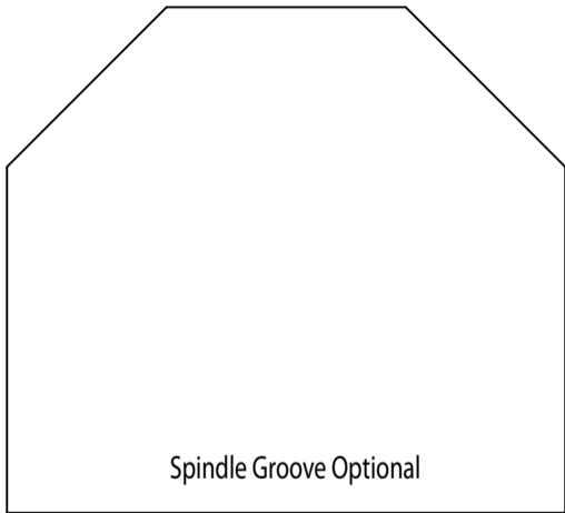
HWP4320 Handrail 2.375" x 2.625"
