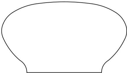
HWP4271 Handrail 1.281" x 2.250"
