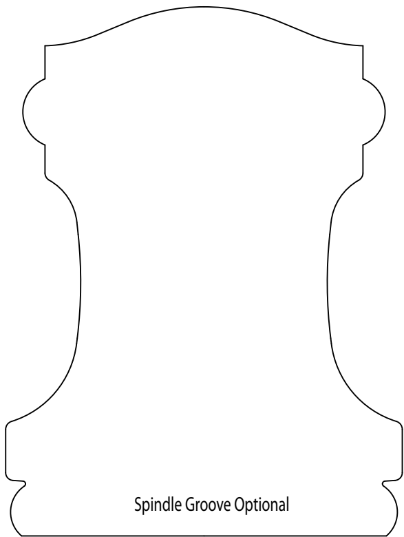
HWP4256 Handrail 4.000" x 3.000"
