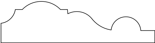
HWP4080 Chair Rail 0.750" x 2.750"
