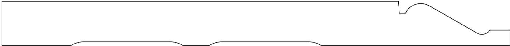
HWP3532 Base 0.750" x 8.500"
