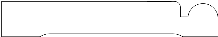
HWP3261 Base 0.750" x 4.500"
