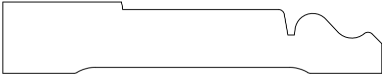
HWP3067 Base 0.750" x 4.000"
