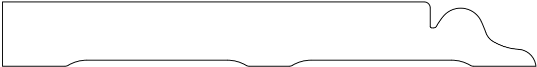
HWP3058 Base 0.665" x Variable
