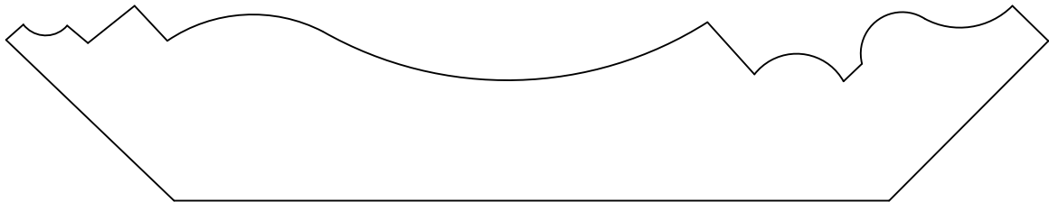
HWP2660 Crown 1.125" x 6.000"
