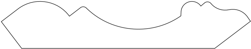
HWP2655 Crown 1.000" x 5.250"
