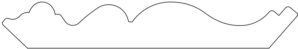
HWP2654 Crown 0.812" x 5.215"
