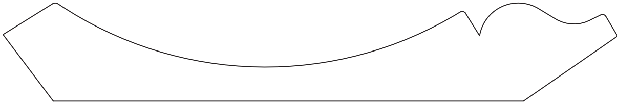
HWP2613 Crown 1.000" x 6.250"
