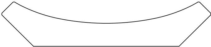
HWP2591 Crown 0.750" x 3.500"
