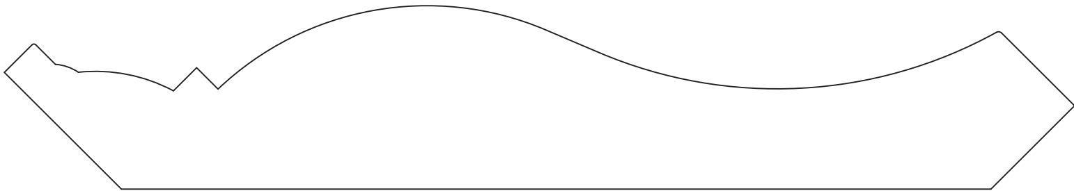
HWP2086 Crown 1.375" x 8.000"
