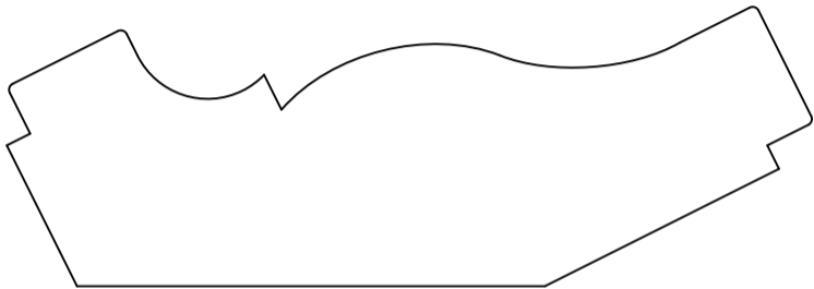
HWP2079 Crown 1.328" X 3.844"
