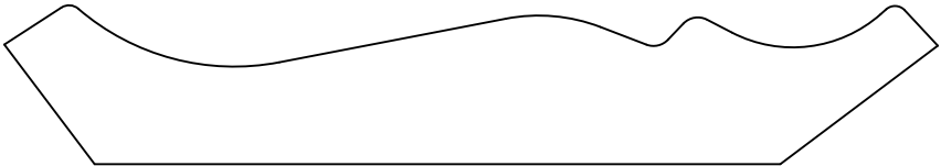
HWP2072 Crown 0.750" x 4.400"
