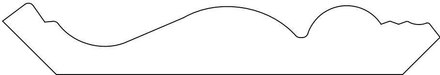
HWP2048 Crown 0.750" x 4.750"
