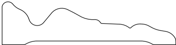
HWP1997 Casing 0.750" x 3.000"
