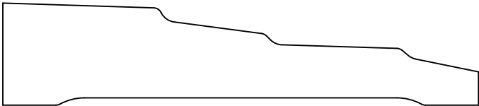
HWP1985 Casing 0.750" x 3.500"
