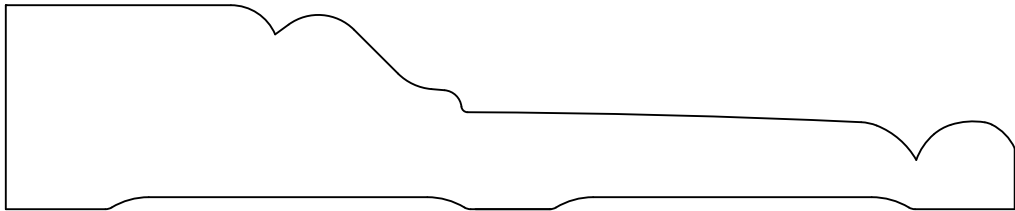
HWP1963 Casing 1.062" x 5.250"
