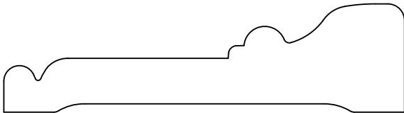
HWP1940 Casing 0.8125" x 3.000"
