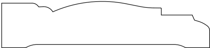
HWP1905 Casing 0.750" x 3.500"
