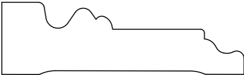
HWP1777 Casing 0.750" x 2.500"
