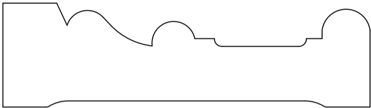
HWP1762 Casing 1.062" x 3.750"
