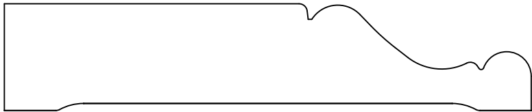
HWP1746 Casing 0.812" x 4.000"
