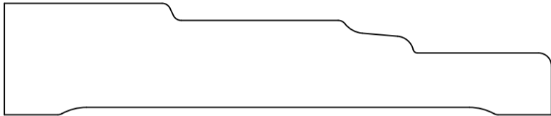
HWP1713 Casing 0.812" x 4.000"
