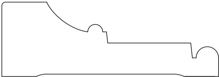
HWP1570 Casing 1.250" x 3.625"
