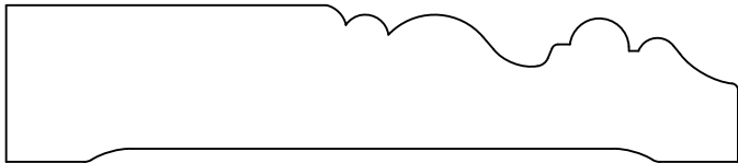
HWP1568 Casing 0.750" x 3.500"
