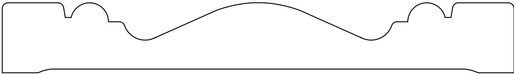
HWP1559 Casing 0.750" x 5.500"
