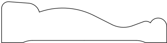
HWP1266 Casing 0.750" x 3.000"
