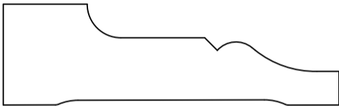
HWP1253 Casing 0.750" x 2.500"
