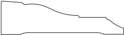
HWP1237 Casing 0.687" x 2.500"
